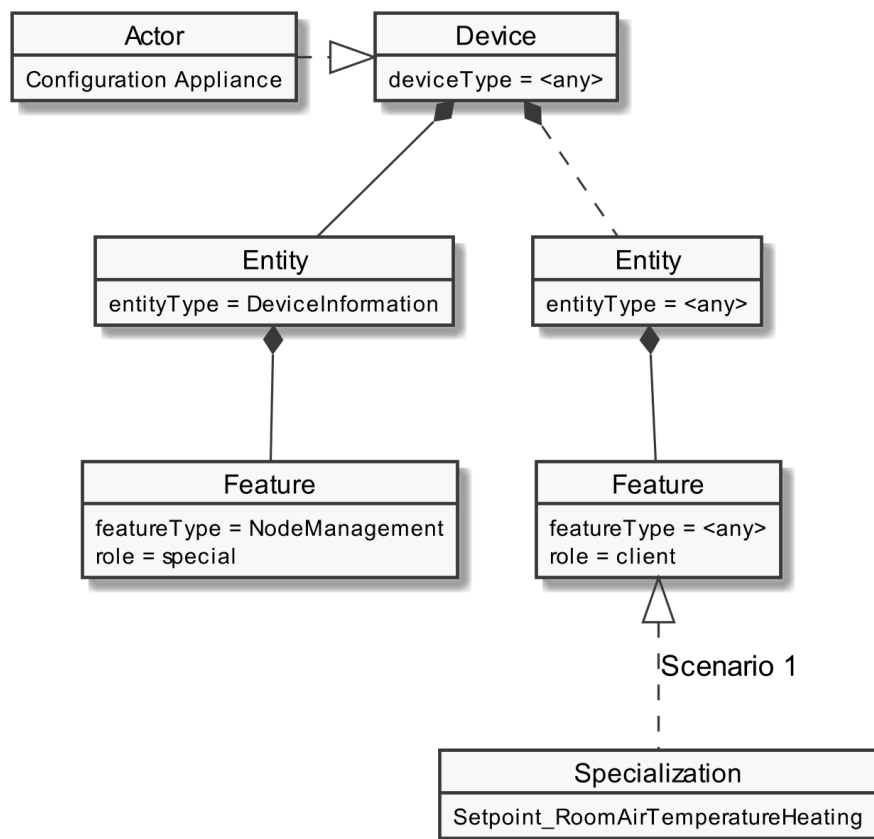
Figure 5: Actor "Configuration Appliance" overview
