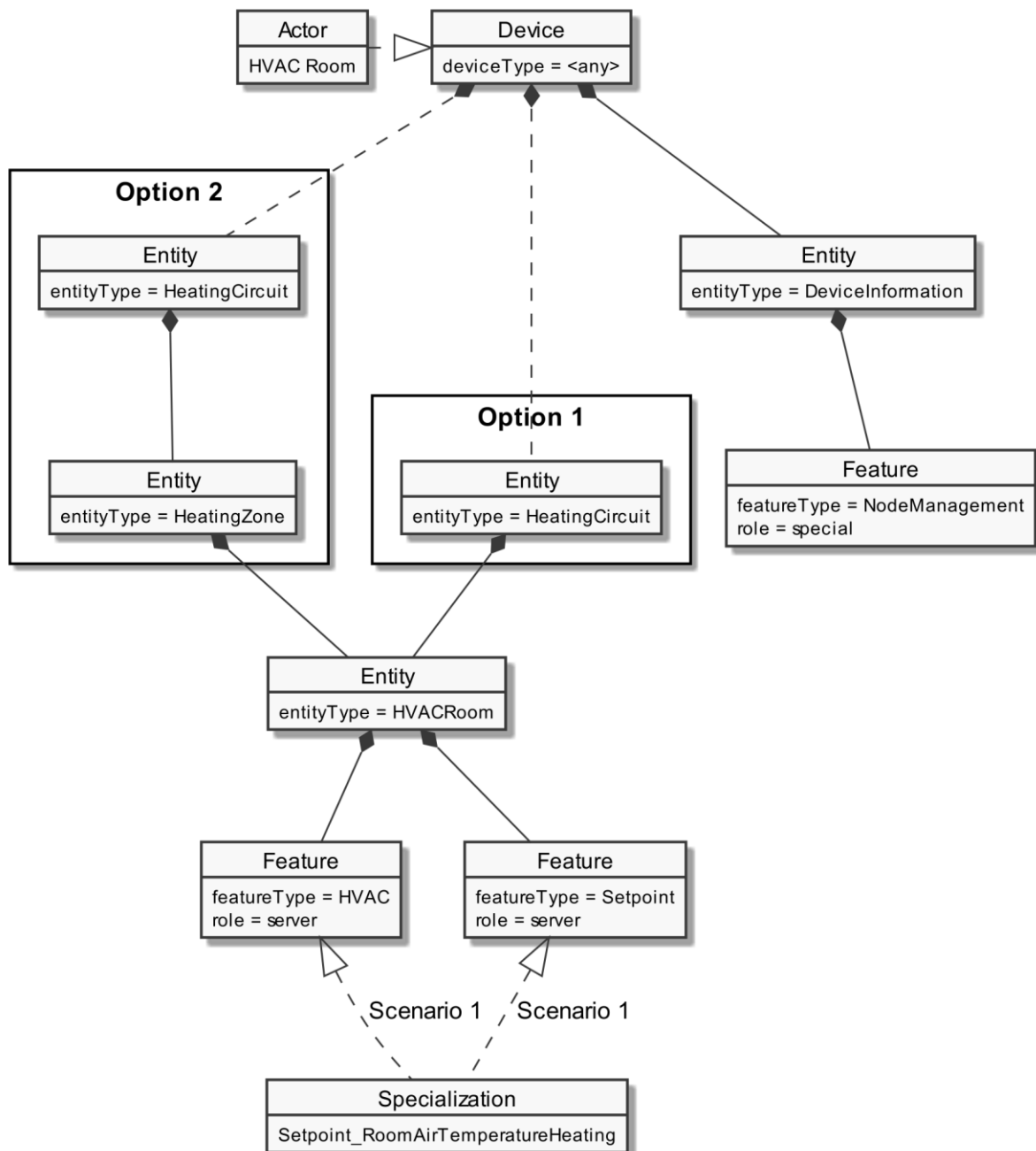
Figure 4: Actor "HVAC Room" overview
